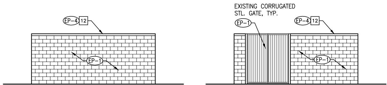
SOUTH ELEVATION
